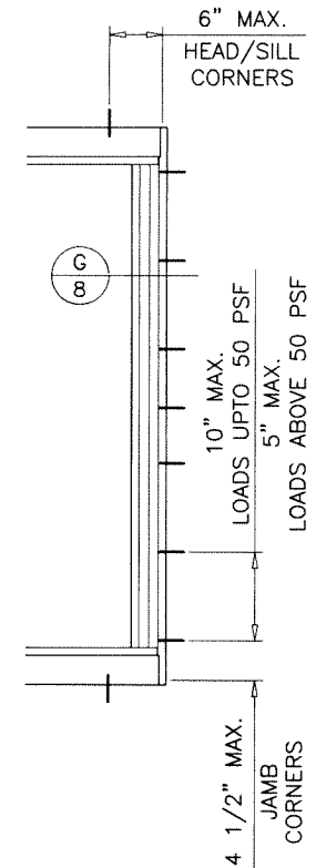
ANCHORED JAMB OPTION
